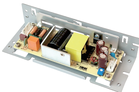
▲ UNBWT1050 Series with chassis
