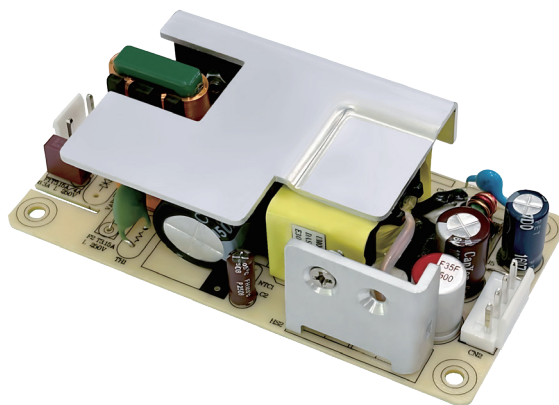
▲ UxOYT3065 Series
